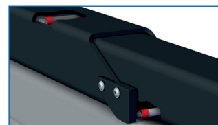
Support arm assist by double roller spring bearing on top/bottom side (MA STAR 5.5/6.5 Comfort – patent pending)
